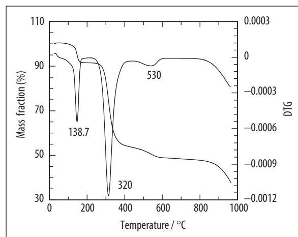
Fig. 7 TG-DTG of ZnO-4CPA nanomaterial shows the appearance of two endothermic bands at 138°C and 320°C.
